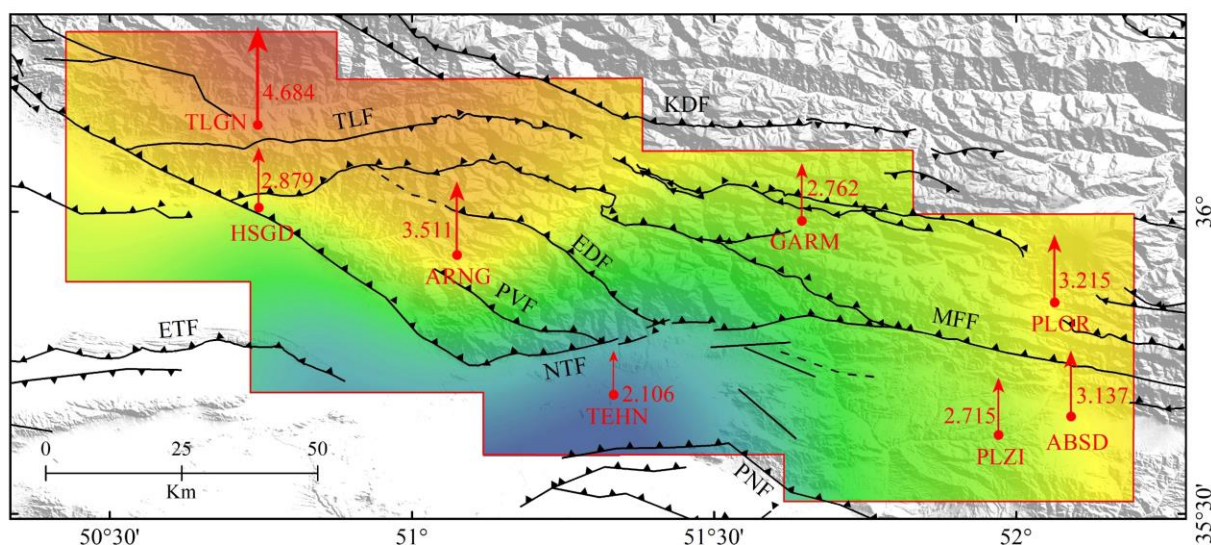
Fig. 2. The heat map resulted from interpolating the height change rate of different IPGN stations superimposed on the SRTM-based digital elevation model.
