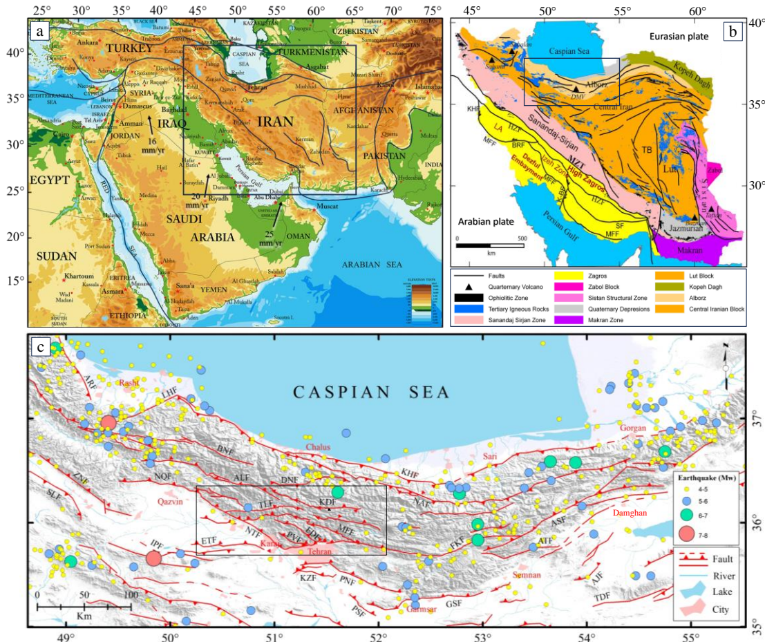
Fig. 1. Geographic and tectonic location of the study area. (a) SRTM-based Digital Elevation Model of the Middle East region. The black lines and the black frame show the main faults and the location of Fig. (b). (b) The structural-sedimentary zones of Iran (taken from Teknik and Ghods, 2017), the black frame shows the location of Fig. (c). (c) Seismotectonic map of northern Iran. Instrumental seismicity of the region from 1900-2024 (from the USGS). The black frames indicate the location of the North Tehran structural zone and surrounding areas. Abbreviations: NTF: North Tehran fault, PVF: Purkan-Vardij Fault, EDF: Emamzadeh Davud Fault, MFF: Mosha-Fasham Fault, TLF: Taleghan Fault, KDF: Kandovan Fault, DNF: Dasht-e-Nazir Fault, NAF: North Alborz Fault, KHF: Khazar Fault, BNF: Banan Fault, LHF: Lahijan Fault, ARF: Astara Fault, NQF: North Qazvin Fault, ALF: Alamut Fault, ZNF: Zanzan Fault, SLF: Soltanieh Fault, IPF: Ipak Fault, ETF: Eshtehard Fault, KZF: Kahrizak Fault, PNF: Parchin Fault, PSF: Pishva Fault, GSF: Garmsar Fault, FKF: Firuzkuh Fault, ATF: Atari Fault, ASF: Astaneh Fault, AJF: Anjilu Fault, TDF: Torud Fault.
