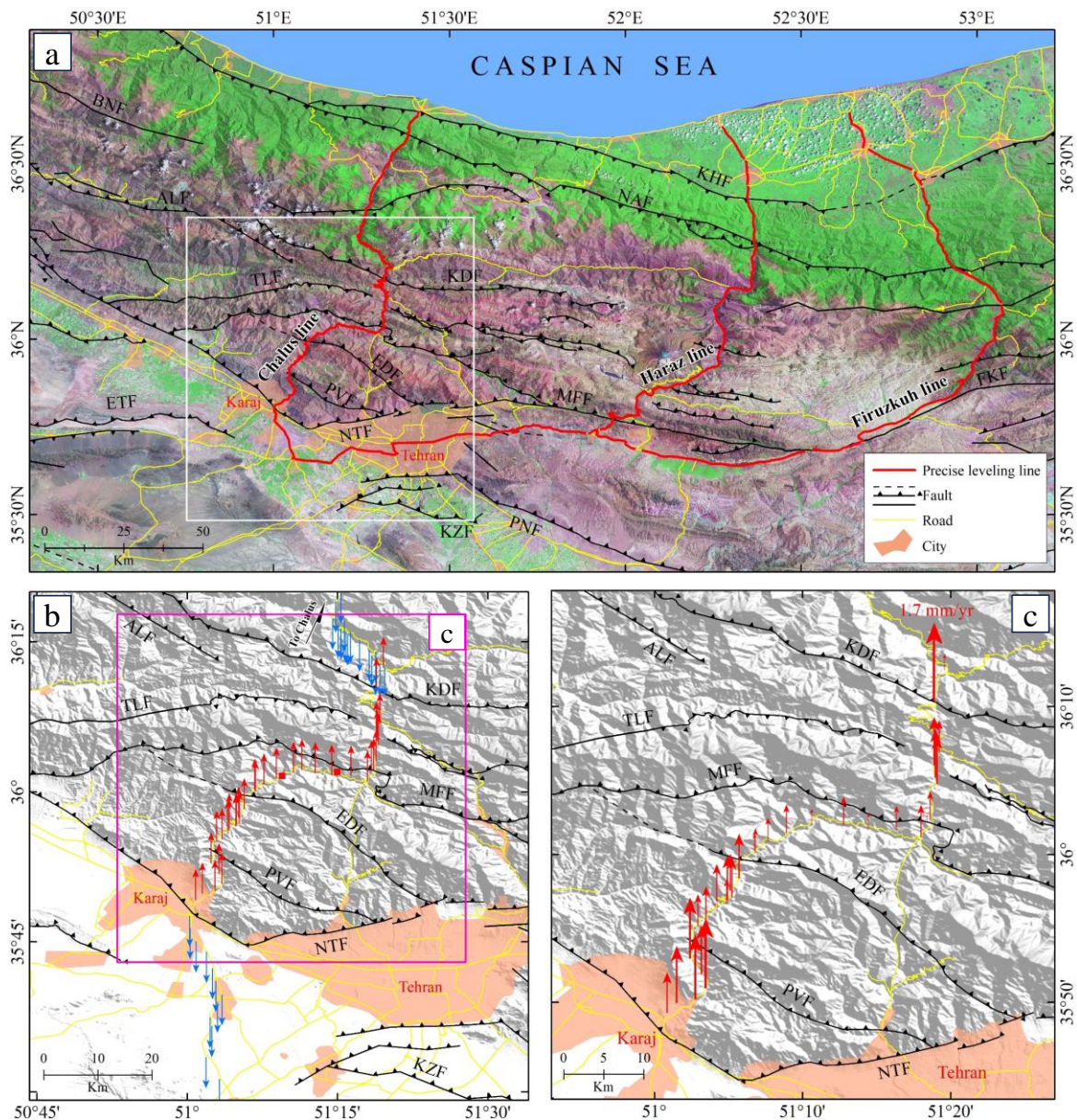
Fig. 3. (a) location of the Chalus, Haraz, and Firuzkuh lines (red lines), which have precise leveling stations along themselves superimposed on the Mr. SID satellite imagery of central Alborz. The Chalus line passes through the middle parts of the North Tehran structural zone. The white frame shows the location of Fig. (b). (b) Superimposing precise leveling stations on the SRTM-based digital elevation model. The red and blue arrows, without respecting the scale, show the uplift and subsidence, respectively, at the location of the precise leveling stations. The purple frame represents the location of Fig. (c). (c) Illustration of uplift rate calculated at precise leveling stations between North Tehran and Kandovan faults. Abbreviations are the same as in Fig. 1.
