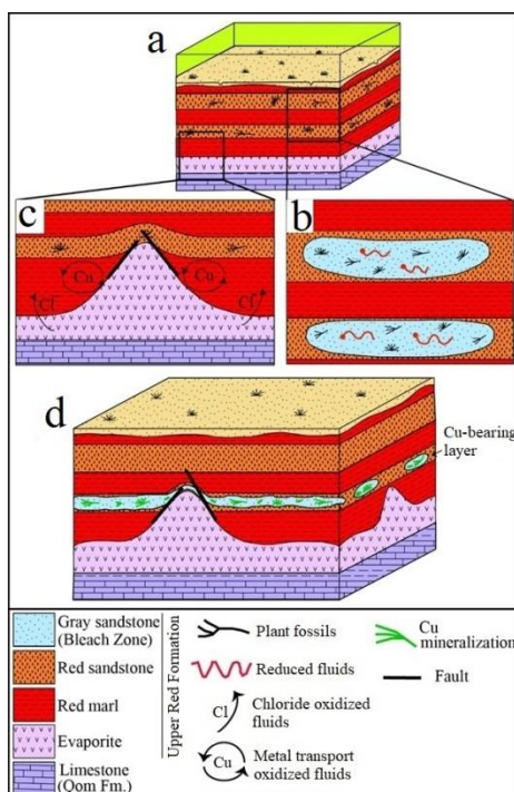
Fig. 10. Schematic diagram showing tectonic setting and sedimentary environment of the Upper Red Formation in the Hamzelou area at Pre-mineralization stage (Ghasemlou, 2018).
